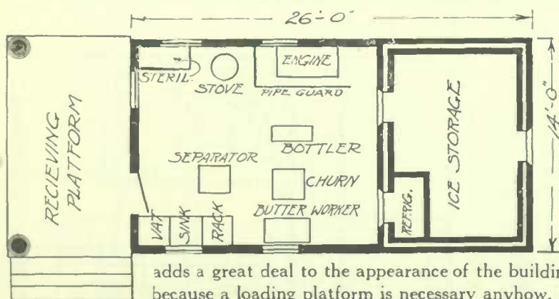
Design 2600C — Creamery
