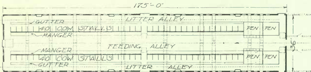
Design 2603 — For 80 Cows
