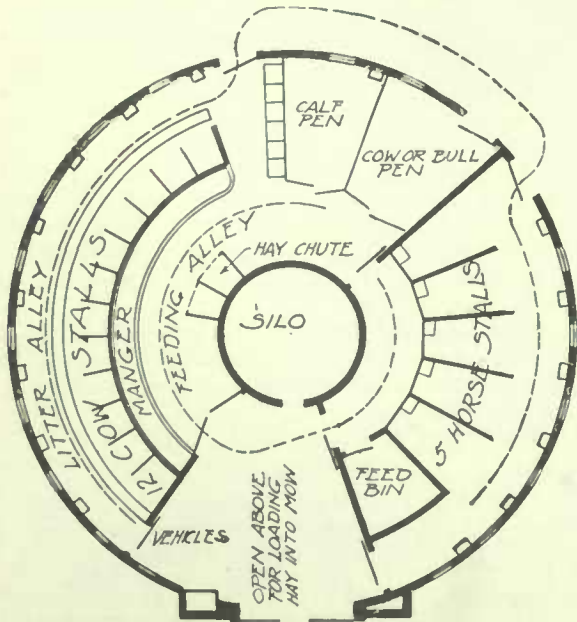
Design 2868—For 12 Cows and 5 Horses
