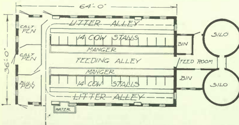
Design 3133—For 28 Cows
