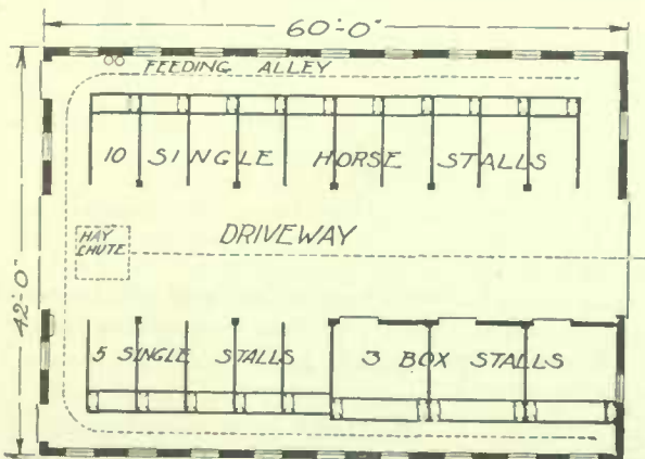
Design 2448—For 18 Horses
