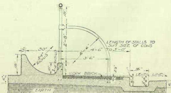
Section of Louden Cow Stall
