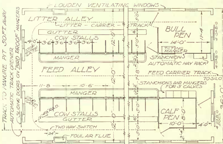
Typical Plan of Dairy Barn
