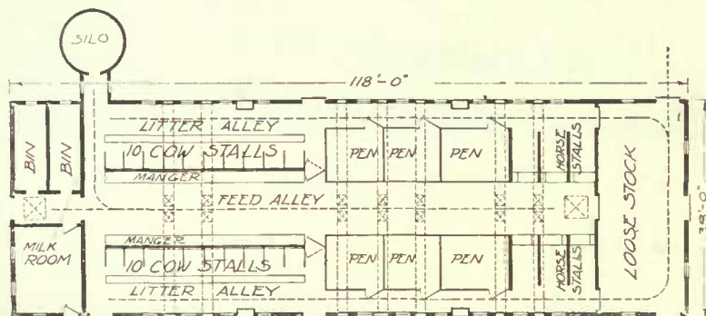
Design 2569 — For 20 Cows and 6 Horses
