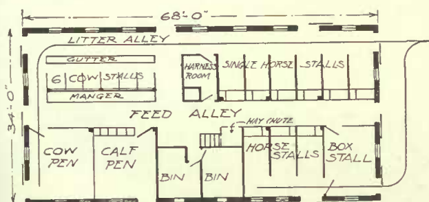
Design 1797—For 6 Cows and 10 Horses
