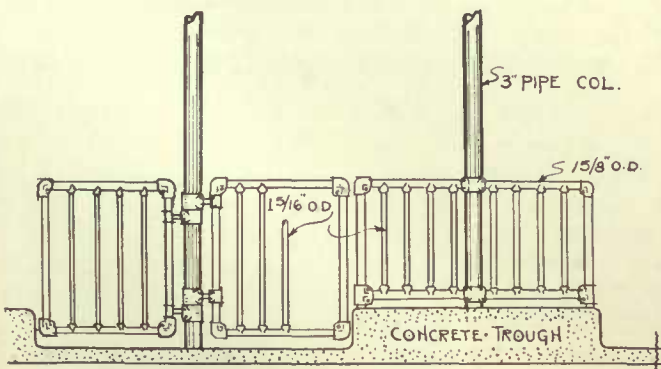
FRONT · PANEL
