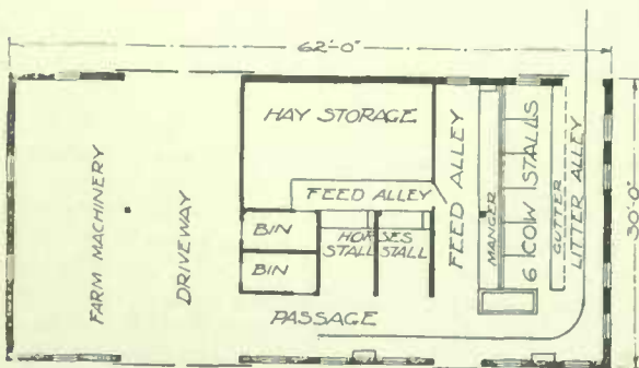
Design 2067—For 6 Cows and 2 Horses
