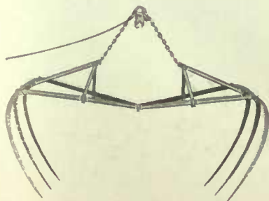
Louden Balance Grapple Fork.
