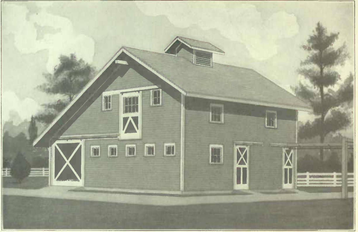
Design 2420 — For 4 Cows and 4 Horses
