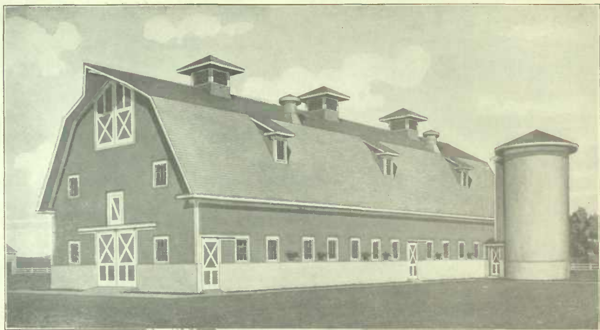
Design 2569 — For 20 Cows and 6 Horses
