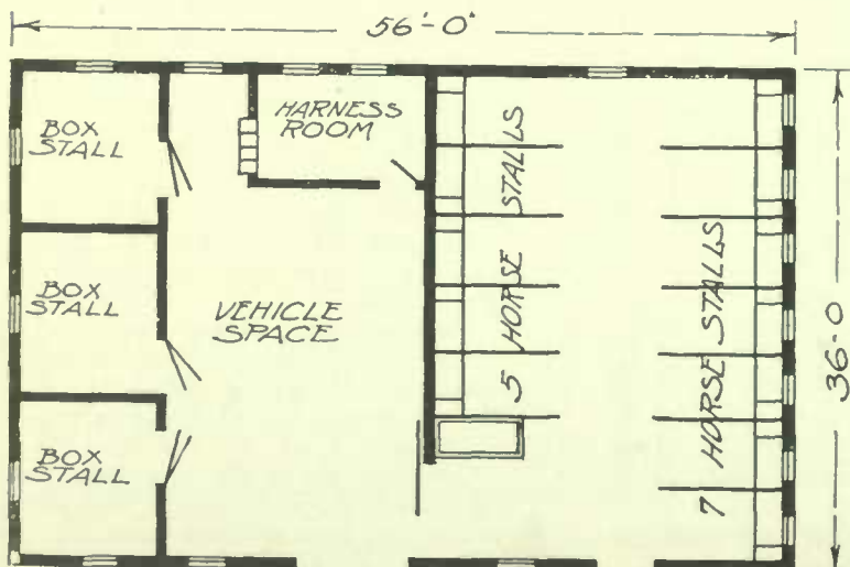
Design 2600A—Horse Barn
