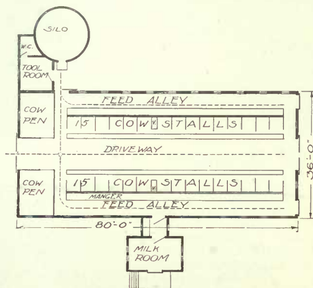
Design 2419—For 30 Cows
