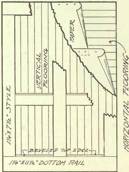
EXTERIOR ELEVATION OF DOORS
