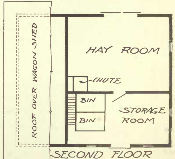
Design 2420 — For 4 Cows and 4 Horses
