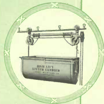
Track arranged with slight incline so carrier may be emptied with trip rope and returned to barn. A barn in Sweden.
