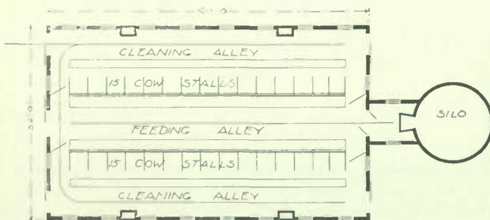
Design 2140—For 30 Cows
