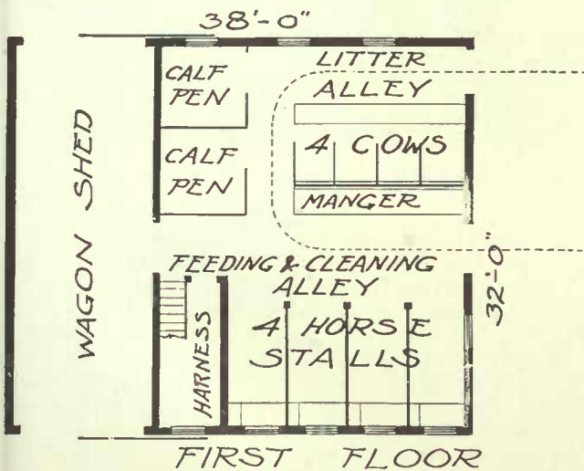
Design 2420 — For 4 Cows and 4 Horses
