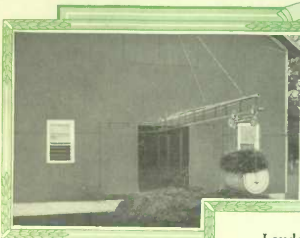
Louden Swinging Cranes are Hinged at barn, making possible a large dumping area, and doing away with posts in the yard.
