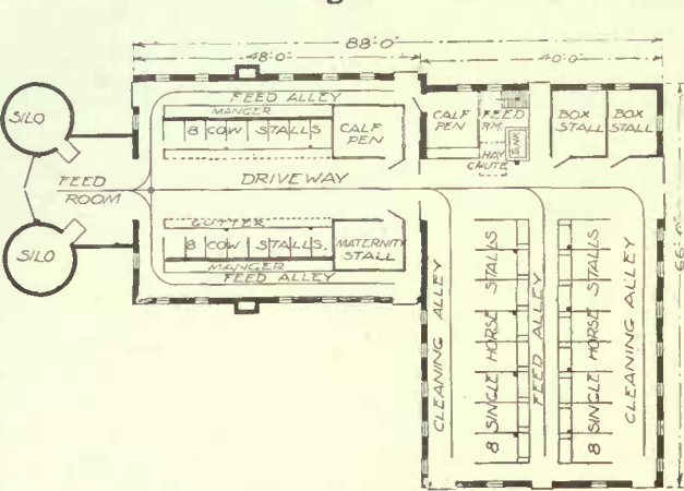
Design 2026—For 16 Cows and 18 Horses
