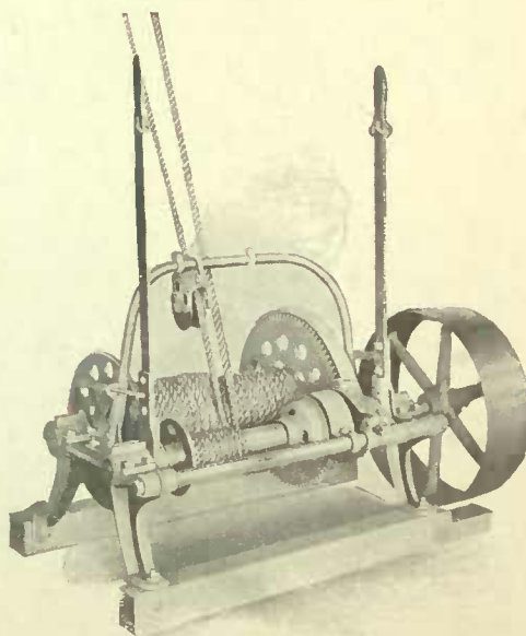
Louden Double Drum Power Hoist.
