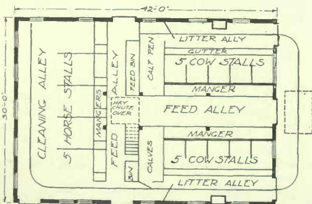
Design 1508—For 10 Cows and 5 Horses
