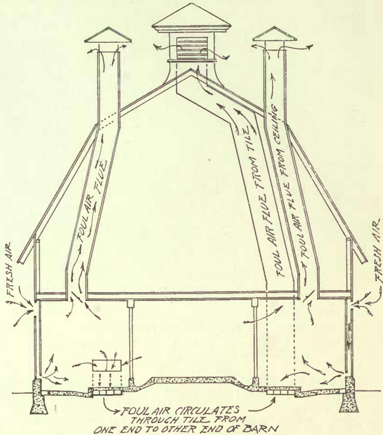
CROSS SECTION SHOWING VENTILATION
