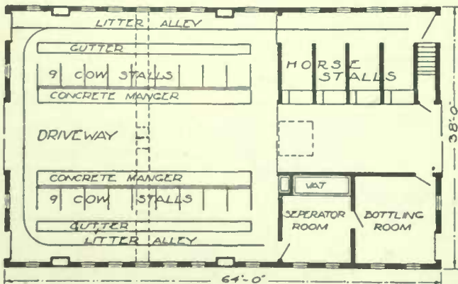
Design 2162—For 18 Cows and 4 Horses
