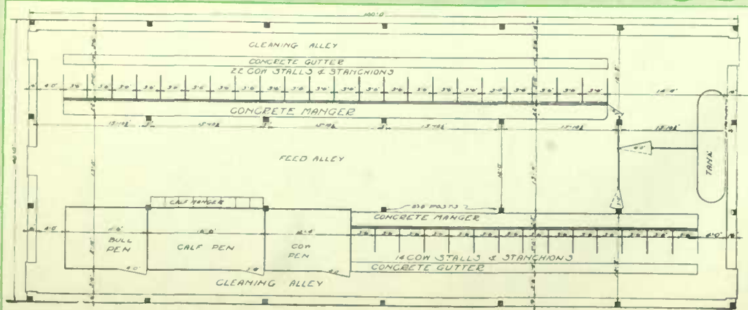
"Tobacco River Ranch"— owned by W. C. Cornwell, Clare, Michigan. This dairy barn was designed by the Loudon Architectural Department and equipped with Cow Stalls, (Fig. 812) Maternity Pens, Calf Pens, and Bull Pen, Emanci- pator Litter Carrier, Double End Feed Carrier, etc. Mr. Cornwell is one of Michigan's progressive dairymen and is giving special attention to breeding pure bred stock.
