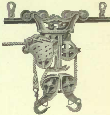
Louden Junior Sling Carrier.
