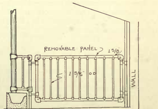
PARTITION · PANEL
