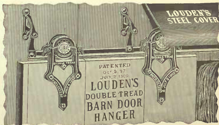
Louden Double Tread Barn Door Hanger.
