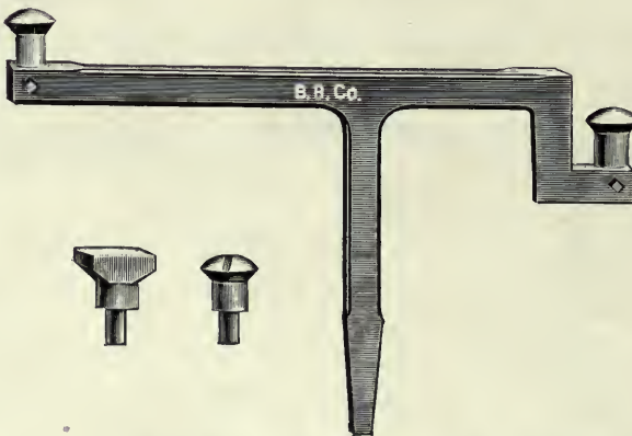
Tea Kettle Stake with 4 Steel Heads
