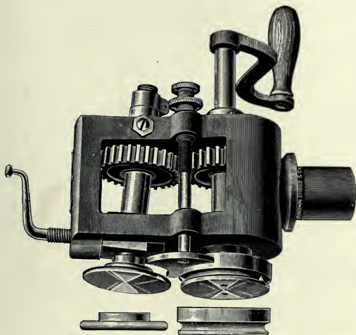
Solid Frame Large Turner
