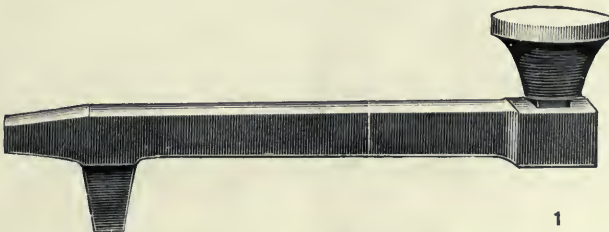
Double Seaming Stake with Four Heads
