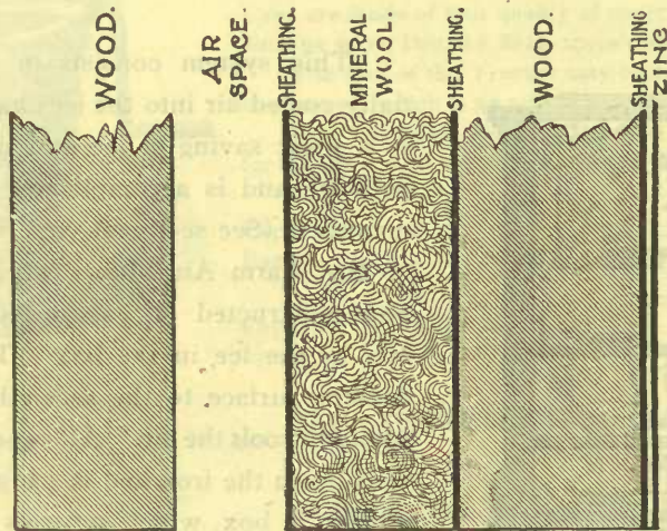
Full size sectional view of one wall of a Leonard Cleanable Refrigerator.
