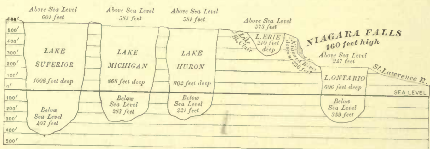
DEPTHS AND LEVELS OF THE GREAT LAKES.
