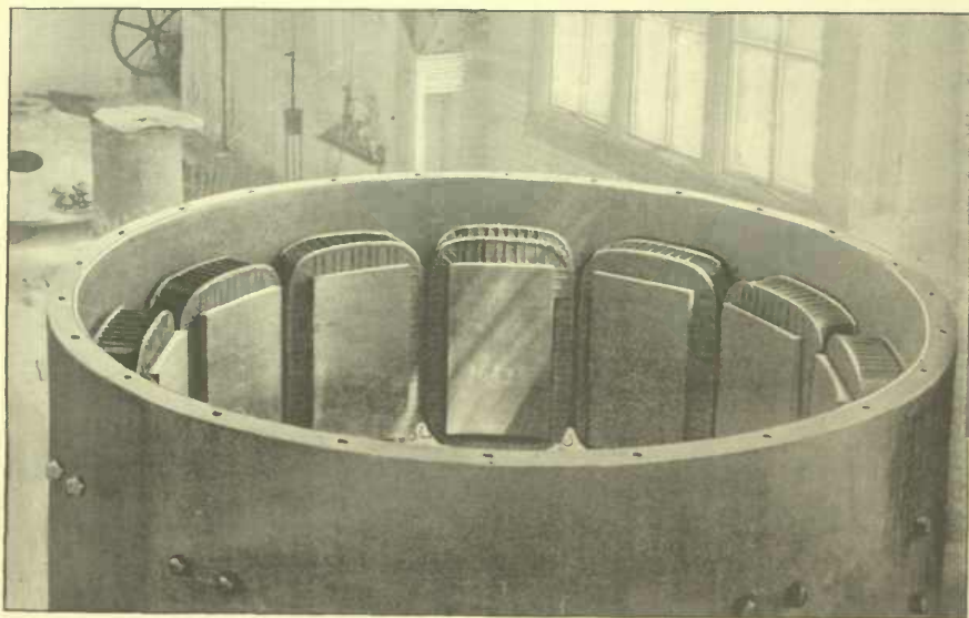
FIELD RING WITH POLES AND BOBBINS IN PLACE.
