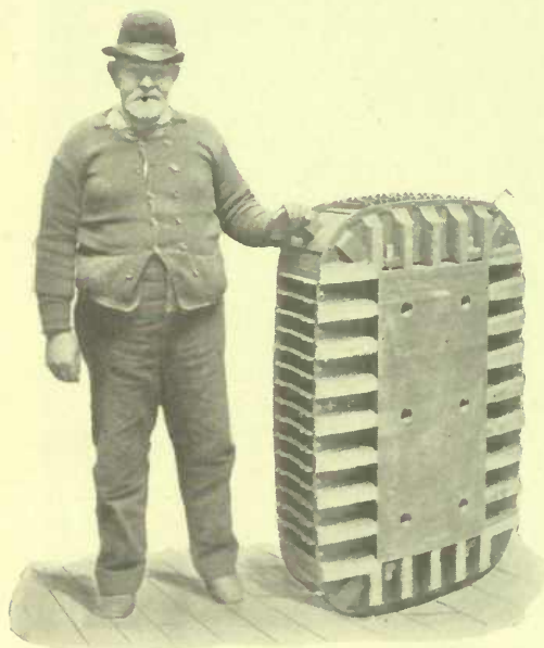
A FIELD POLE WITH WINDING IN PLACE. WEIGHT, 2800 LBS.
