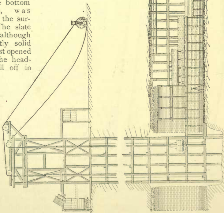
LONGITUDINAL SECTION, SHOWING METHOD EMPLOYED IN SINKING SHAFT, AND TIMBERING, BRICK-LINING AND DRIVING THE MAIN TUNNEL.
