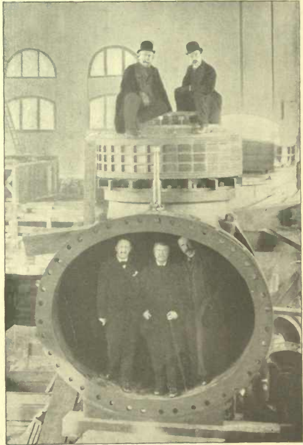
PENSTOCK CONNECTION WITH TURBINE.
