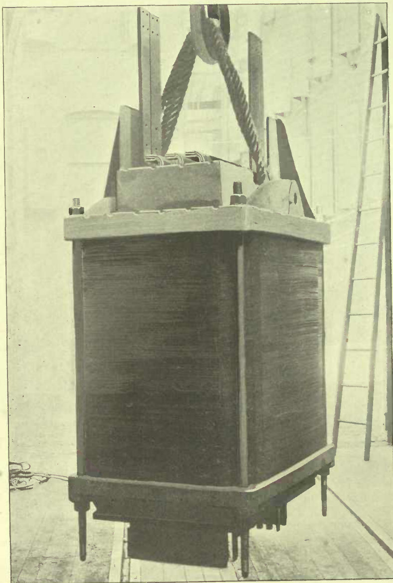
THE INTERNAL MAKE-UP OF THE CARBORUNDUM CO.'S LARGE STATIC TRANSFORMER. THIS TRANSFORMER REDUCES THE PRESSURE OF THE TWO-PHASE ALTERNATING CURRENT FROM 2400 TO 200 VOLTS.
