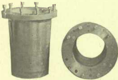
DETAILS OF ARMATURE BEARINGS.
