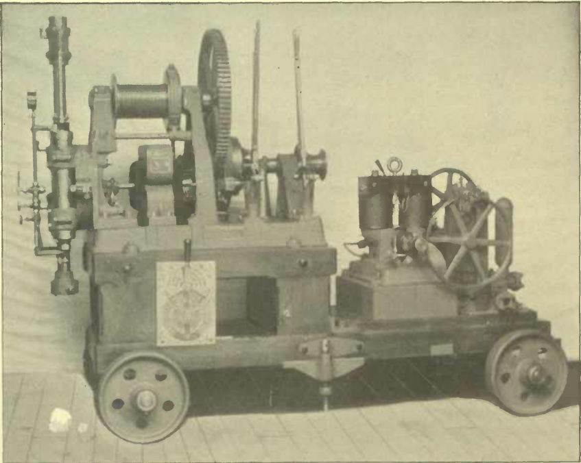
AN ELECTRIC DIAMOND DRILL FOR PROSPECTING WORK.
