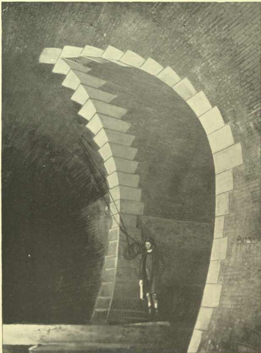
A LATERAL TUNNEL JUNCTION.
