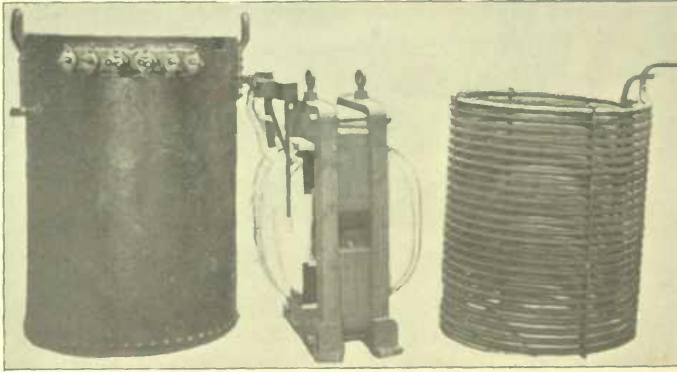
DETAILS OF THE 100 KILOWATT STEP-DOWN TRANSFORMER.
