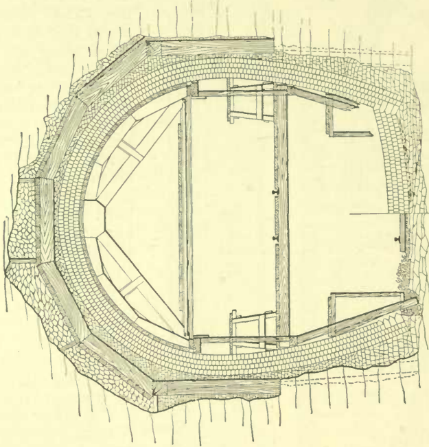
CROSS SECTION OF TUNNEL, SHOWING METHOD OF LINING.
