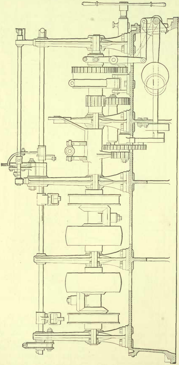
SECTIONAL VIEW OF GOVERNOR. FAESCH & PUCCARD DESIGN.
