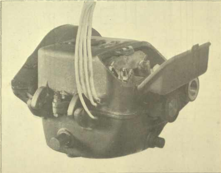
A TYPICAL ELECTRIC STREET CAR MOTOR. 25 HORSE-POWER.
