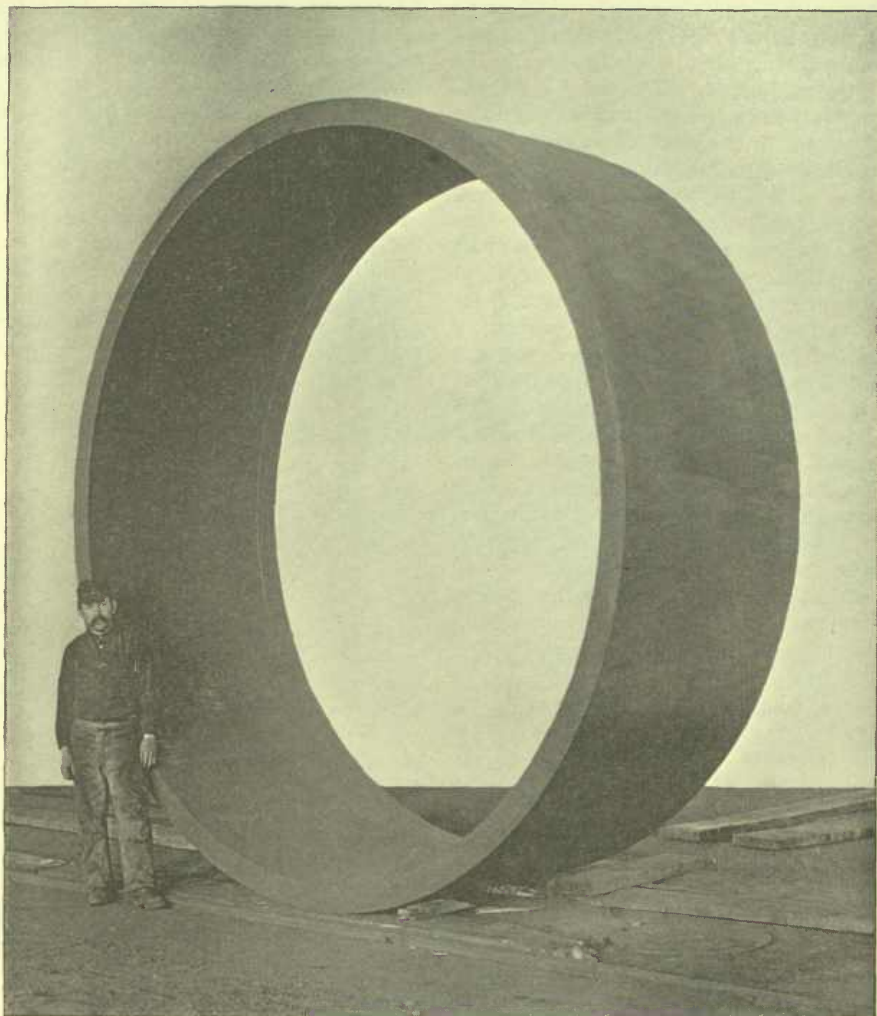
NICKEL STEEL FIELD RING, FORGED WITHOUT A WELD BY THE BETHLEHEM IRON COMPANY. DIAMETER, 11 FT. 7 \frac{1}{8} IN.
