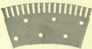
ONE OF THE SHEETS MAKING UP THE ARMATURE CORE.
