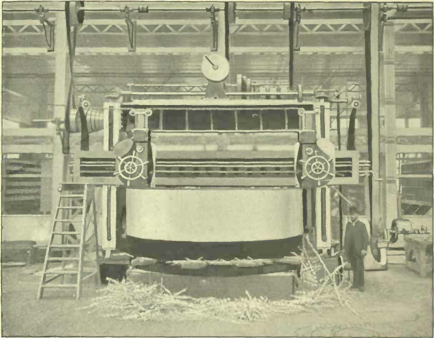
TURNING THE FIELD RING IN THE WESTINGHOUSE SHOPS.
