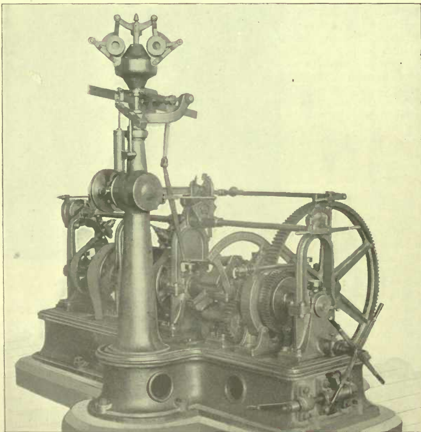
THE FAESCH & PICCARD GOVERNOUR IN PLACE.
