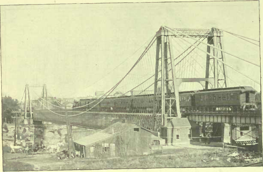
THE NIAGARA FALLS RAILWAY SUSPENSION BRIDGE.
