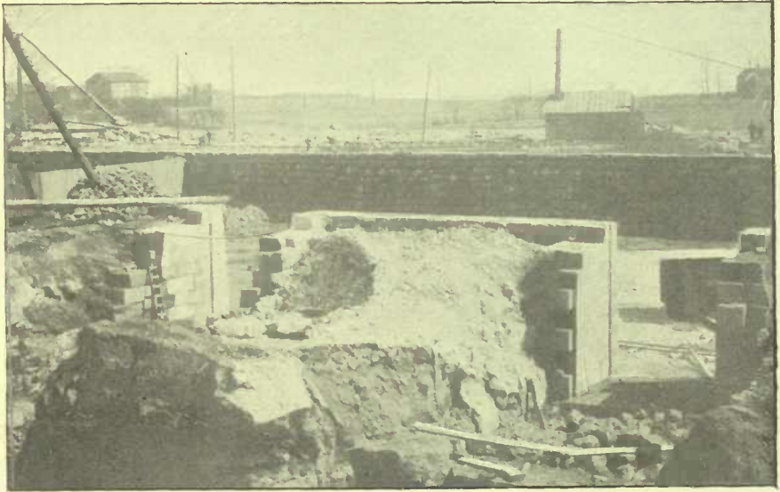
A PROGRESS VIEW OF THE CANAL.
