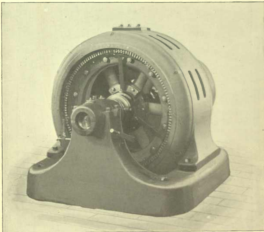
A TYPICAL ALTERNATING CURRENT INDUCTION MOTOR OF 125 HORSE-POWER.
