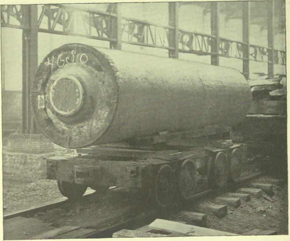
SOLID INGOT OF FLUID COMPRESSED STEEL USED FOR MAKING THE FORGED FIELD RING. LENGTH, 197 IN. DIAMETER, 54 IN. WEIGHT, 120,000 LBS.
