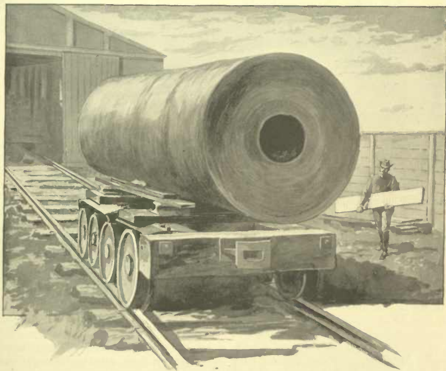
COMPRESSED STEEL INGOT WITH HOLE THROUGH CENTER, PREPARATORY TO FORGING.
