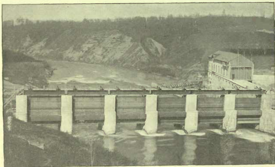
THE STONEY DAM NEAR GENEVA, BUILT IN 1895.
