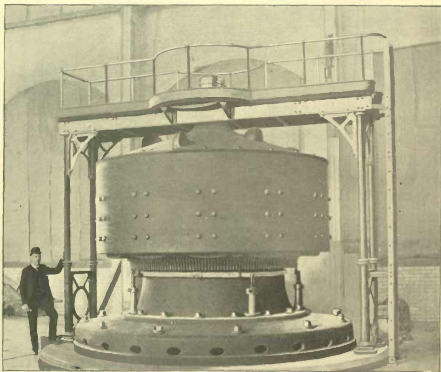
THE FIRST GENERATOR IN POSITION IN THE POWER HOUSE AT NIAGARA.
