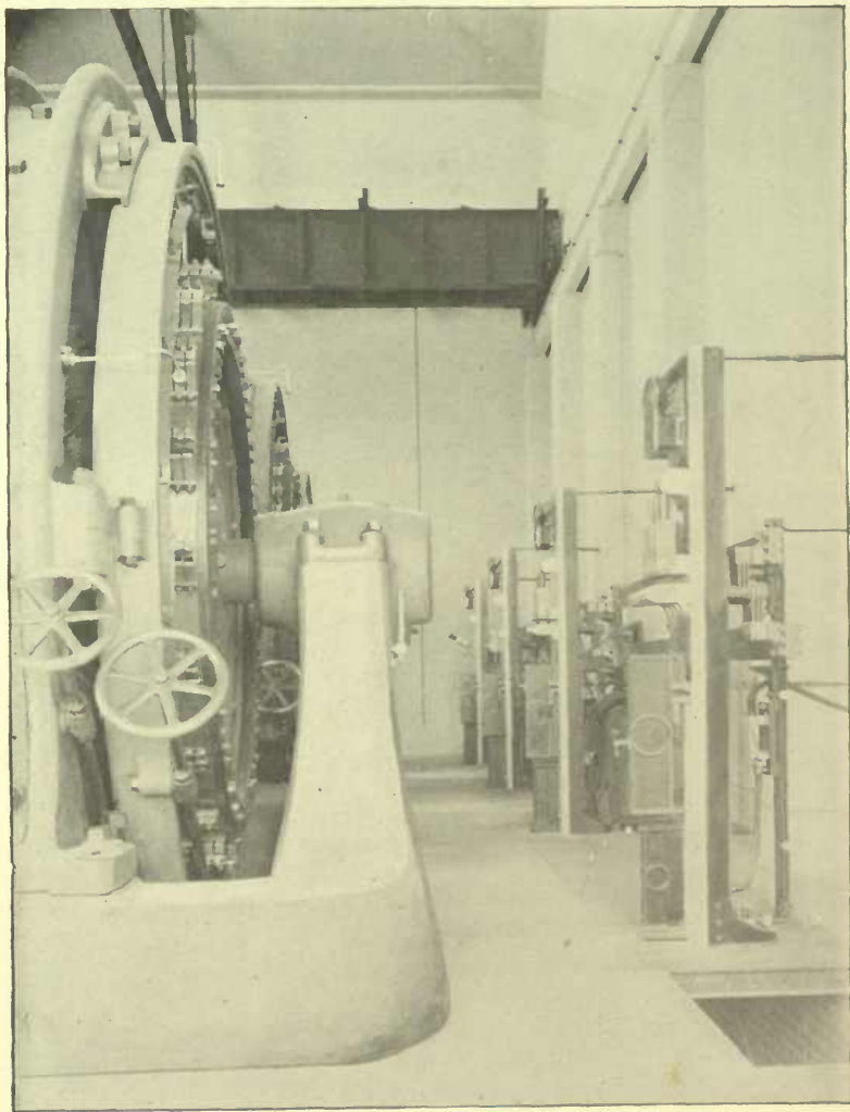
DIRECT-CURRENT SIDE OF THE ROTARY CONVERTERS AND THE LOW-TENSION SWITCHBOARDS.
