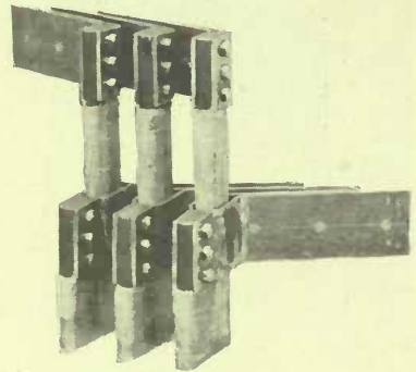
JUNCTION OF ARMATURE BARS AND CONNECTORS BEFORE SOLDERING AND INSULATING.
