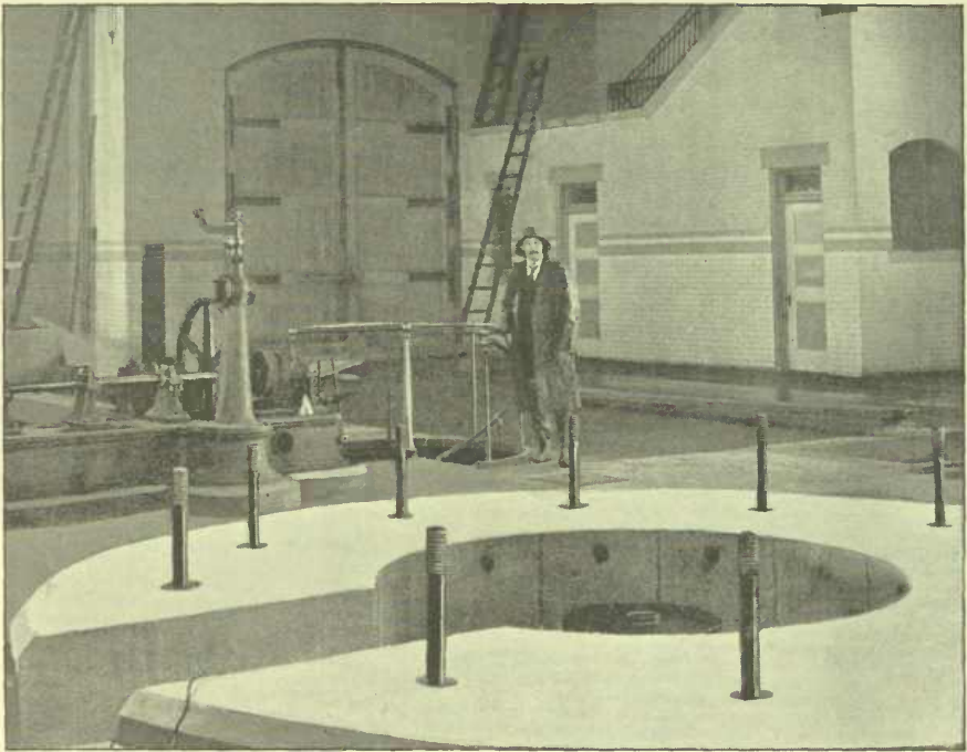
ONE OF THE GENERATOR FOUNDATIONS.
