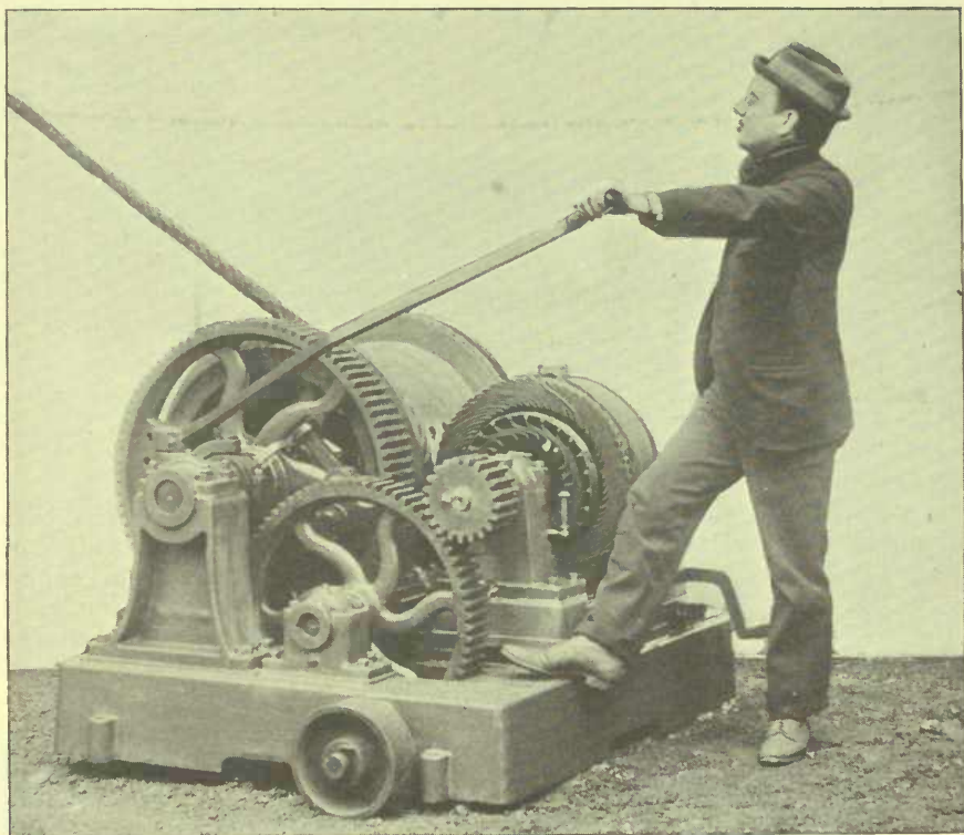
AN ALTERNATING CURRENT INDUCTION MOTOR, GEARED TO A HOIST.
