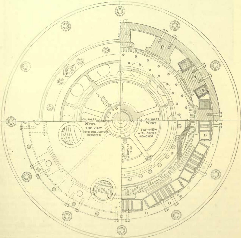
HORIZONTAL SECTION.
