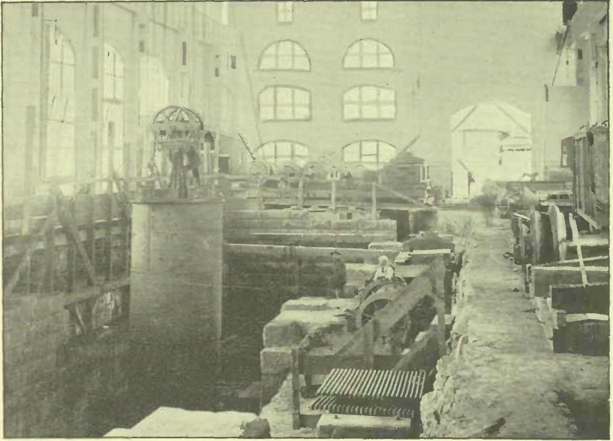
LOWERING A PENSTOCK INTO THE WHEEL-PIT.
