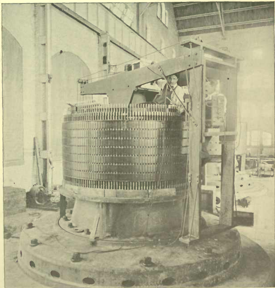
ELECTRICALLY SOLDERING THE CONNECTIONS OF AN ARMATURE WINDING.
