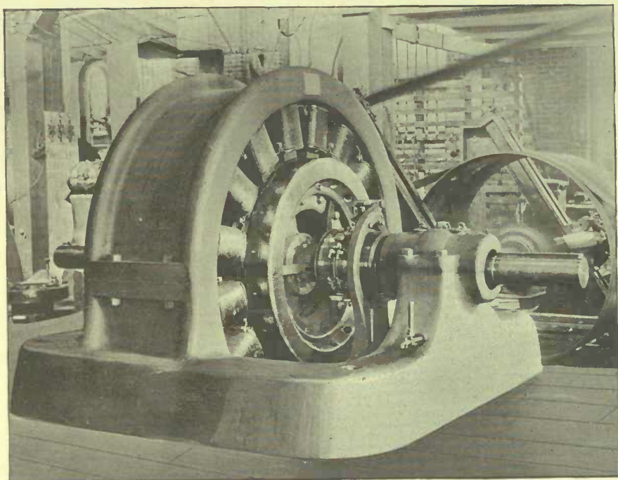
A 250 HORSE-POWER THREE-PHASE ALTERNATING CURRENT MOTOR.
