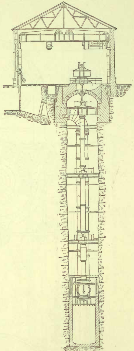
GENERAL ELEVATION OF FAESCH & PICCARD DESIGN.
