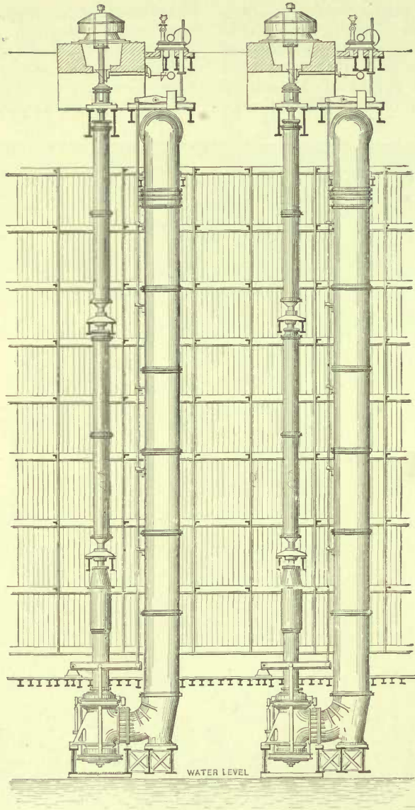
GENERAL ELEVATION. FAESCH &amp; PICCARD DESIGN.
