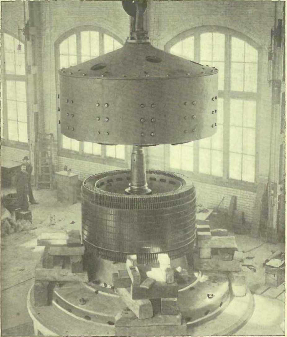
A FIELD RING READY TO BE LOWERED ON A GENERATOR SHAFT.
