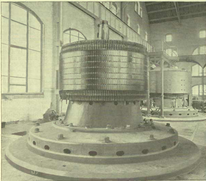
THE ARMATURE OF THE SECOND GENERATOR IN PLACE.
