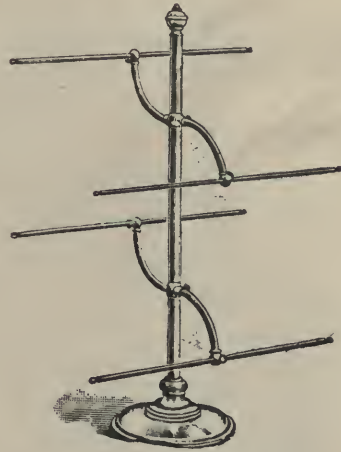
No. 168.—Glove Stand. 6 inch base, \frac{5}{8} inch standard, 2\frac{1}{2} feet high, four \frac{1}{4} x 24 inch rods, set in sliding collars. Nickel plated. Price.... .....$5.35.
