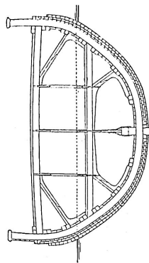
Fig. 3. Transverse section amidships.
