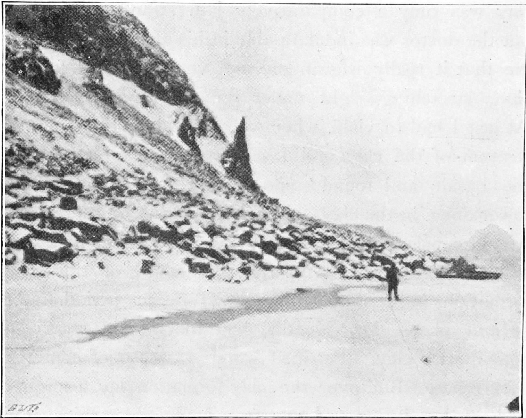
BASALTIC ROCK.
