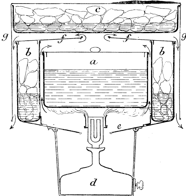
THE COOKING APPARATUS.
