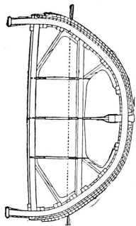
Fig. 3. Transverse section amidships.
