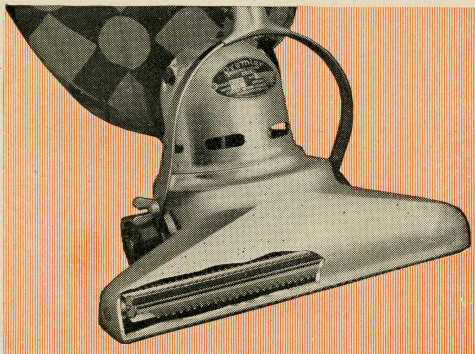
Sectional view showing Revolving Rubber Brush
