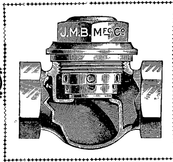
J.M.T. CUSHION CHECK VALVE.
