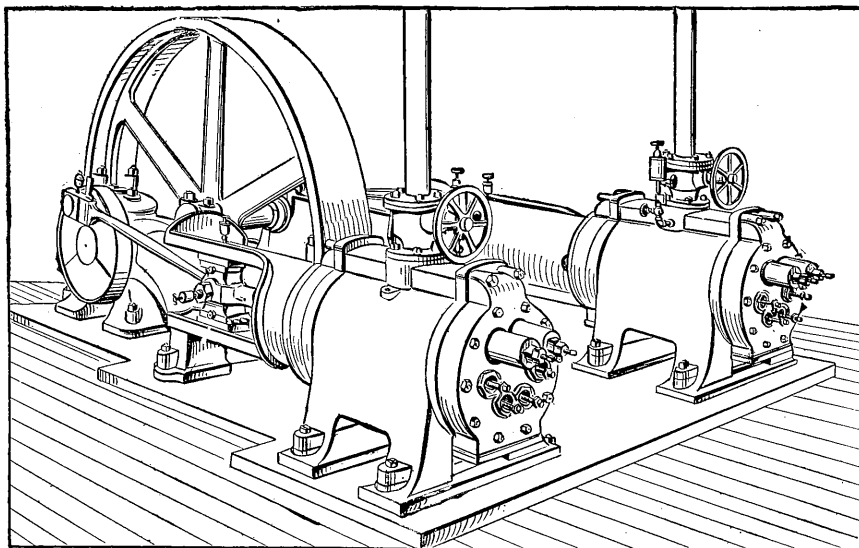
12 x 16 Belt Driven Compressor.
