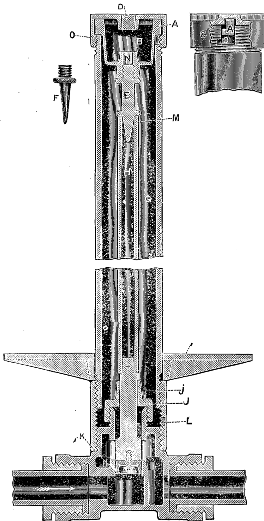
IMPERIAL STOP COCK—Section view showing water cut off.
