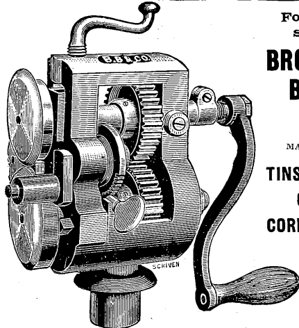
SOLID FRAME SMALL MACHINE.
