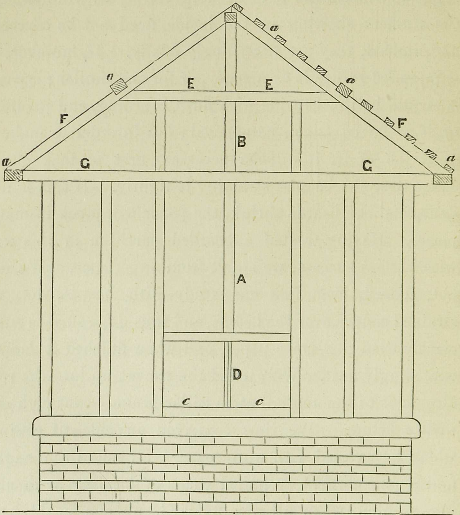
Fig. 15.—Timber Framing.
