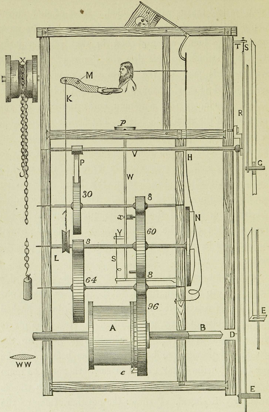
Fig 9.—Clock Train.
