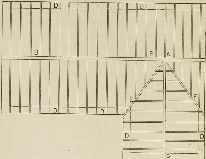
Fig. 17.—Roof Details.
