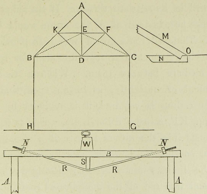
Fig. 16.—Roof Construction.
