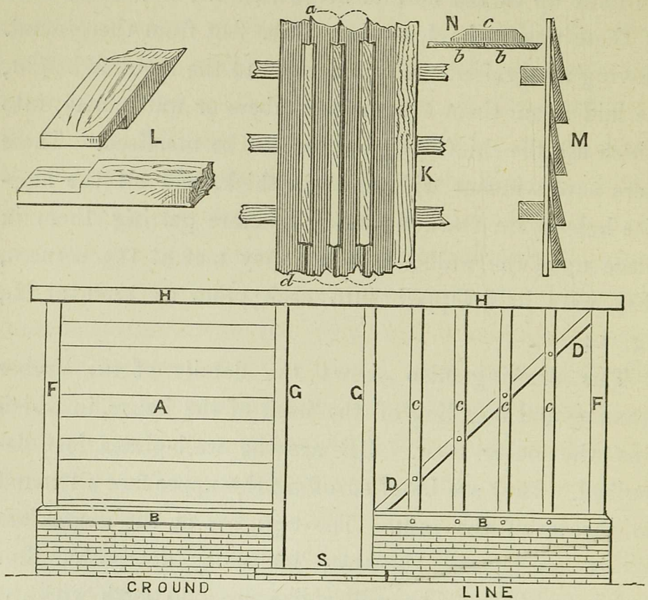
Fig. 14.—House Construction.
