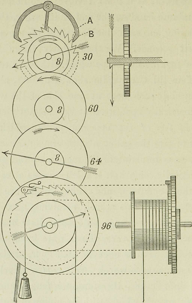
Fig. 7.—Clock Train.
