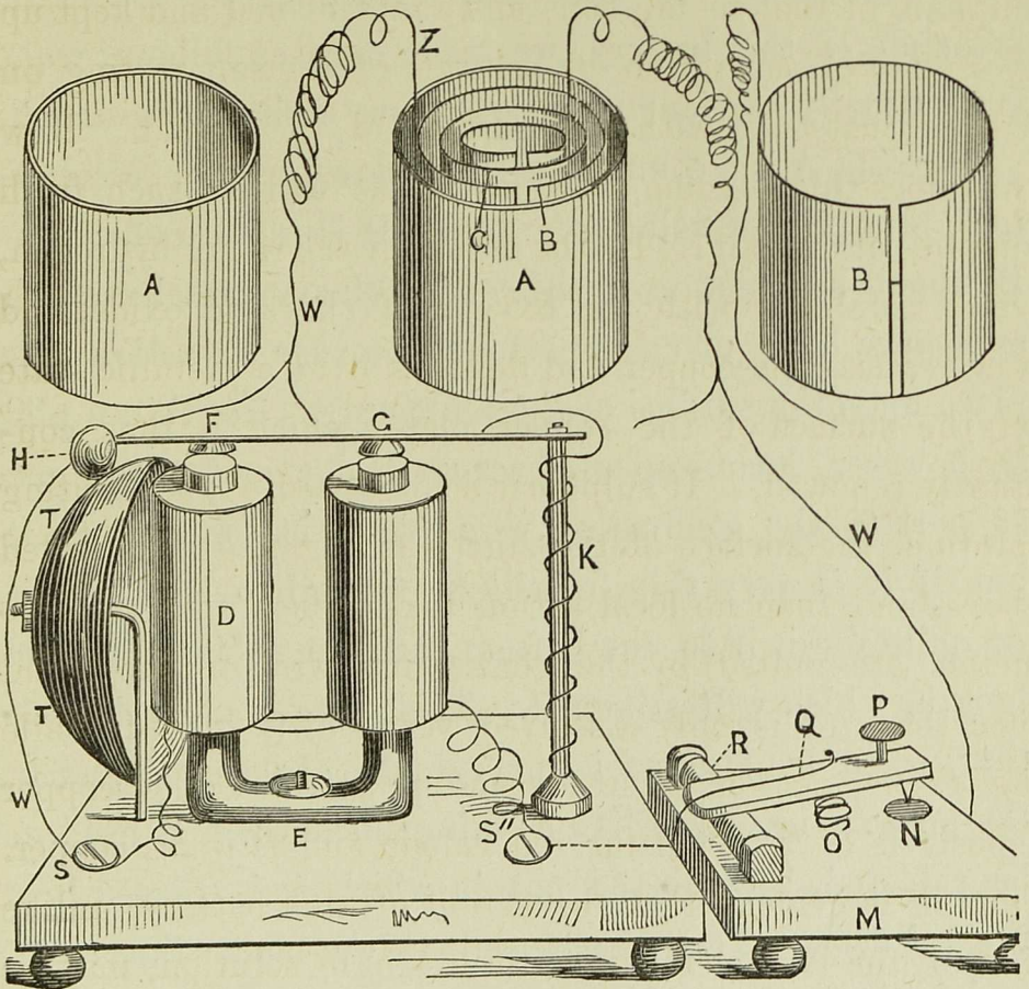
Fig. 26.—Daniell's Galvanic Bell.
