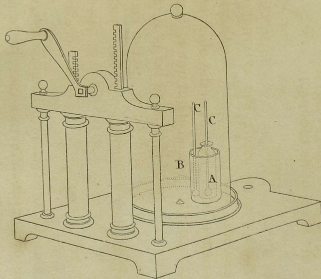
Fig. 1. Pneumatic Pump.
