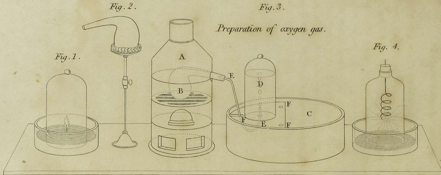
Fig. 1. Combustion of a taper under a receiver.— Fig. 2. A Retort on a stand.— Fig. 3. A Furnace. B Earthen Retort in the furnace. C Water bath. D Receiver. E.E Tube conveying the gas from the Retort through the water into the Receiver. F.F.F Shelf perforated on which the Receiver stands. Fig. 4. Combustion of iron wire in oxygen gas.
