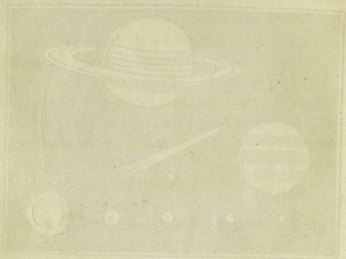
Relative sizes of the planets.
