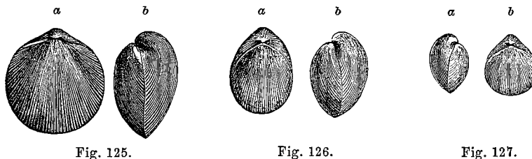
Fig. 125.— Athyris Headi . a , dorsal view; b , side view of a specimen of the typical form. Fig. 126.— a , dorsal view; b , side view of a specimen from Lake St. John (var. A. borealis ). Fig. 127.— a , dorsal view; b , side view of a specimen from Anticosti var. A. anticostiensis ).
