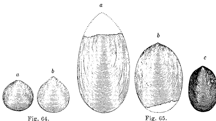
Fig. 64.— Lingula Irene .— a . Specimen found in a boulder of magnesian limestone near Montreal, supposed to be from the calciferous sandrock; b . Specimen from the graptolitic slates, Point Lévis.
