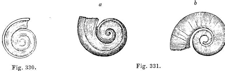
Fig. 330.— Pleurotomaria Arabella . View of the spire.
