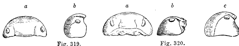
Fig. 319.— Illænus incertus . a , upper side of a perfect head; b , side view of the same.
