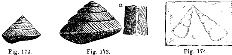
Figs. 172–174.— Pleurotomaria Quebecensis . Fig. 174. A polished section through a specimen, showing the wide umbilicus. a , magnified view of the margin of the body-whorl.
