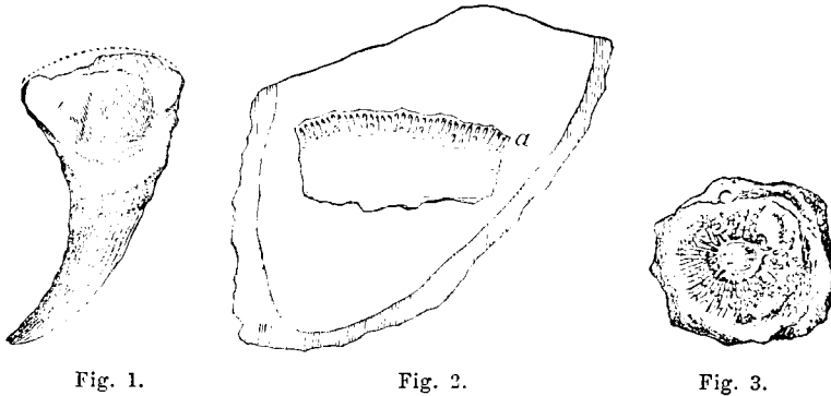
Fig. 1.—The slender base of attachment. Fig. 2.—A longitudinal section through the base of the cup of a worn specimen; a , a transverse section of a fragment where the diameter of the cup is 3\frac{1}{2} inches, showing the radiating septa between the outer and inner walls. Fig. 3.—A transverse section across the base below the bottom of the cup.
