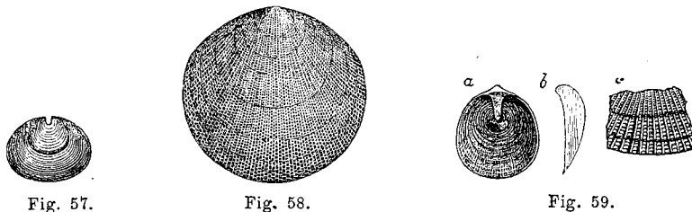
Fig. 57.— Trematis Montrealensis . Lower valve, shewing the small penduncular notch.
