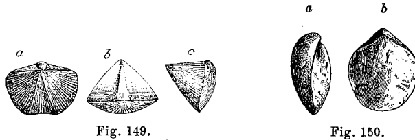
Fig. 149.— Cyrtia Myrtea .— a , Ventral view; b , view of the area; c , side view.
