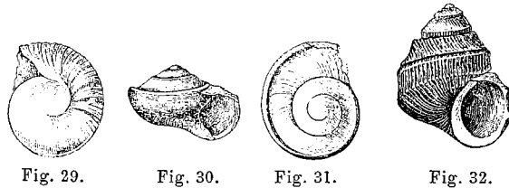
Fig. 29.— Pleurotomaria Eugenia . Fig. 30 view of the underside. Fig. 31 shewing the aperture. Fig. 32.— P. Arachne shewing the spire and band.
