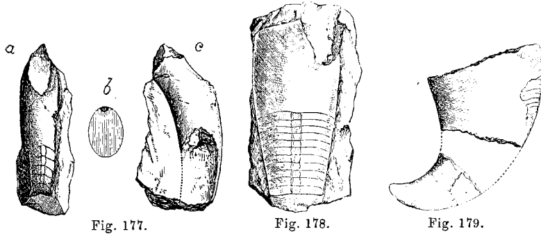
Fig. 177.— Cyrtoceras Alethes . a, ventral view; b, section; c, side. 178.— C. Syphax . Ventral view. 179.— Cyrtocerina Mercurius . Side view.
