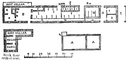
Ground Plan.
