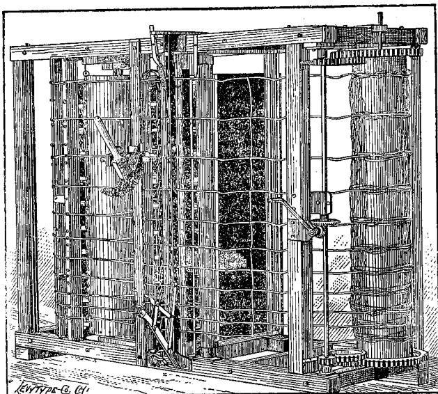
THE AMERICAN WIRE FENCE MACHINE.
