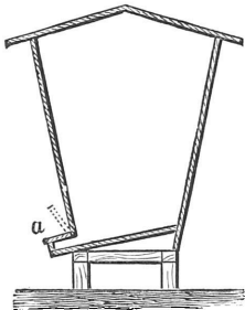
Fig. 138.—SECTION OF CRIB.
