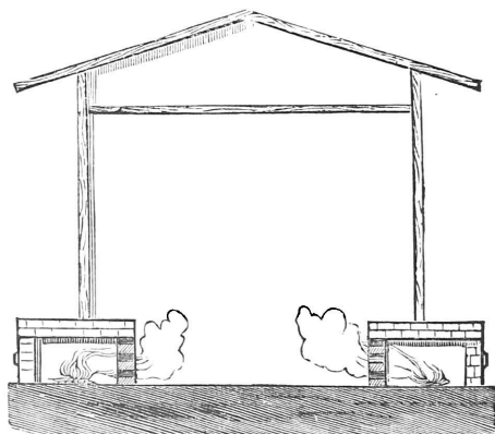
Fig. 196.—WOODEN SMOKE HOUSE WITH OVENS.
