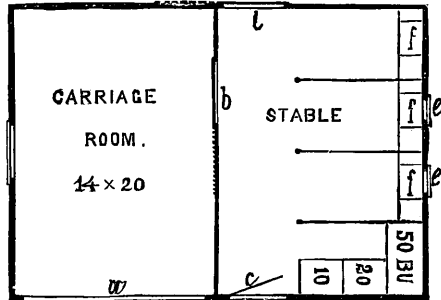
Fig. 25.—GROUND PLAN OF BARN.
