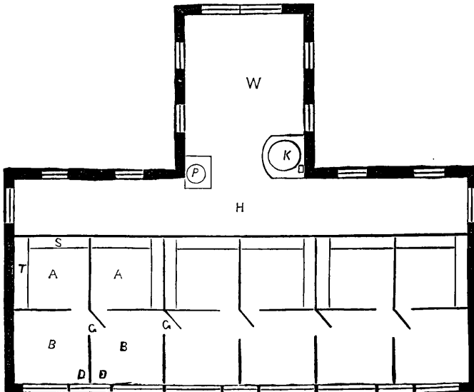
Fig. 101.—GROUND PLAN OF PIGGERY.
