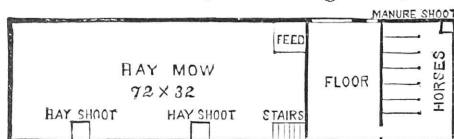
Fig. 54.—PLAN OF MAIN FLOOR.
