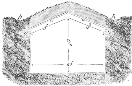
Fig. 236.—CROSS SECTION OF A FIELD ROOT CELLAR.
