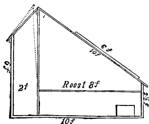
Fig. 92.—SECTION OF HOUSE.
