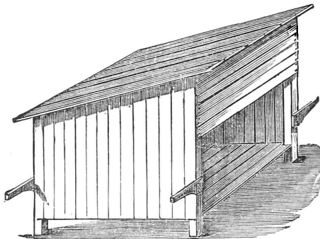
Fig. 115.—A PORTABLE PIGPEN.
