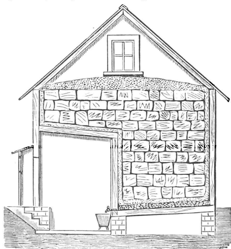
Fig. 160.—ICE HOUSE AND REFRIGERATOR.
