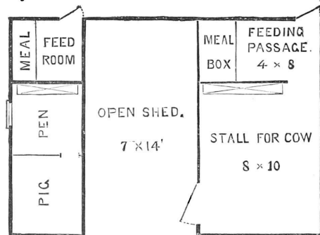
Fig. 48.—PLAN OF COW SHED AND PIGPEN.
