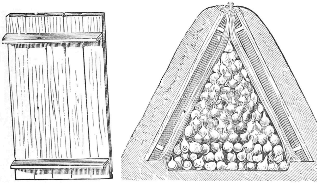
Fig. 238.—SHUTTER FOR PIT. Fig. 239.—SECTION OF FINISHED PIT.
