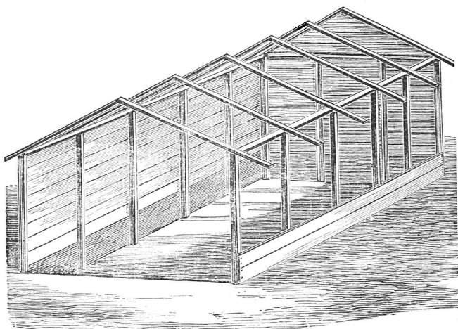
Fig. 141.—A FRAME FOR AN ICE HOUSE.
