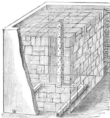
Fig. 168.—ICE HOUSE AND PIPES.
