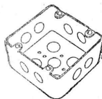
No. 52151—4 in. Sq. Box, 1/2 in. K.O.
