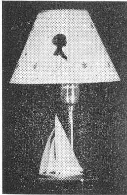
No. 465 —Sailboat. Supplied with Black Glass Base, Metal Sailboat. Shade supplied with Sailboat design to match. Height Overall, 11 in. Dia. of Shade, 7 in.
