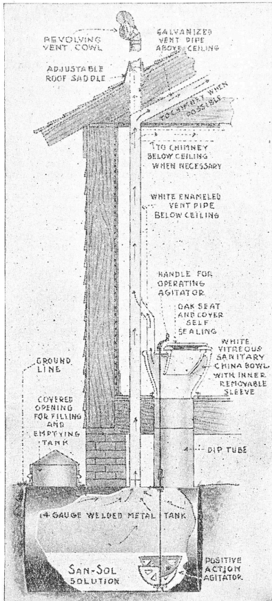
Single Bowl Ground Floor Installation. (Sectional View)
