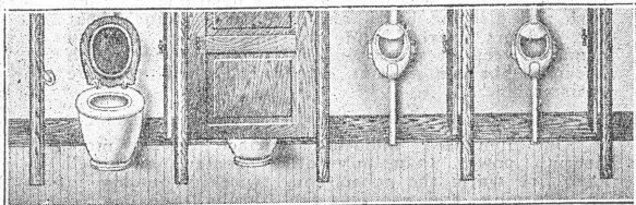
A MULTIPLE INSTALLATION In this case Two Bowls and Two Urinals are installed on a Quadruple Size Tank.
