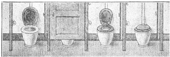
A MULTIPLE INSTALLATION In this case Four Bowls are installed on a Quadruple Size Tank.
