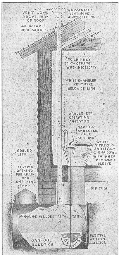
Single Bowl Ground Floor Installation. (Sectional View)
