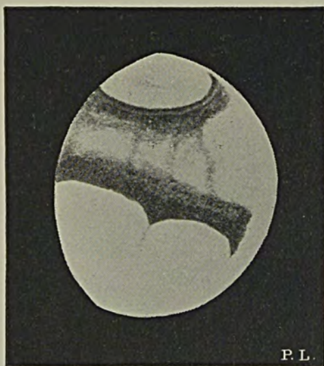
FIG. I. Hesperia at June presentation Long. 242^{\circ} . Lat. centre of disk 24^{\circ} South
