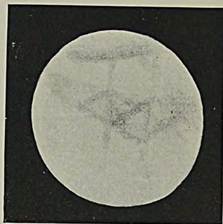
FIG. IV. Dec. 1. Long. cent. 246^{\circ} Seeing 2 to 4. Diam. 14''.9
