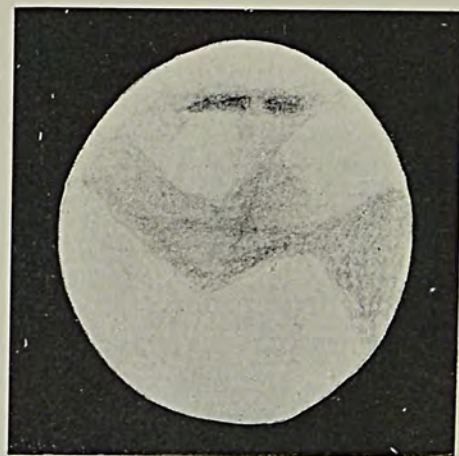
FIG. VI. Jan. 8. Long. cent. 266^{\circ} Seeing 1 to 3. Diam. 9''.9
