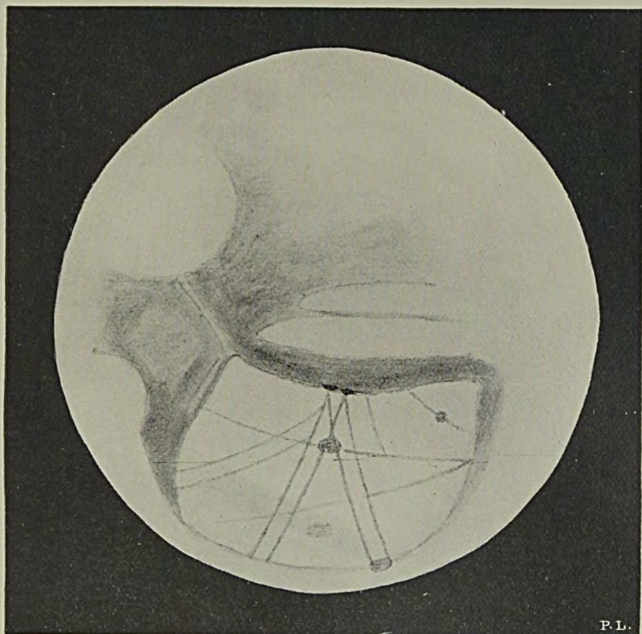
PHISON AND EUPHRATES (Both double) NOVEMBER 18, 1894
