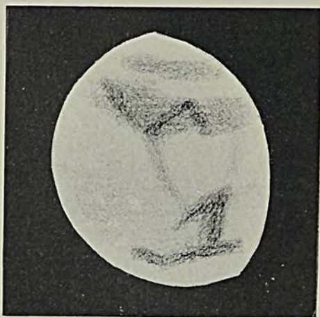
FIG. V. Feb. 21. Long. cent. 193^{\circ} Seeing 2 to 4. Diam. 7''.4
