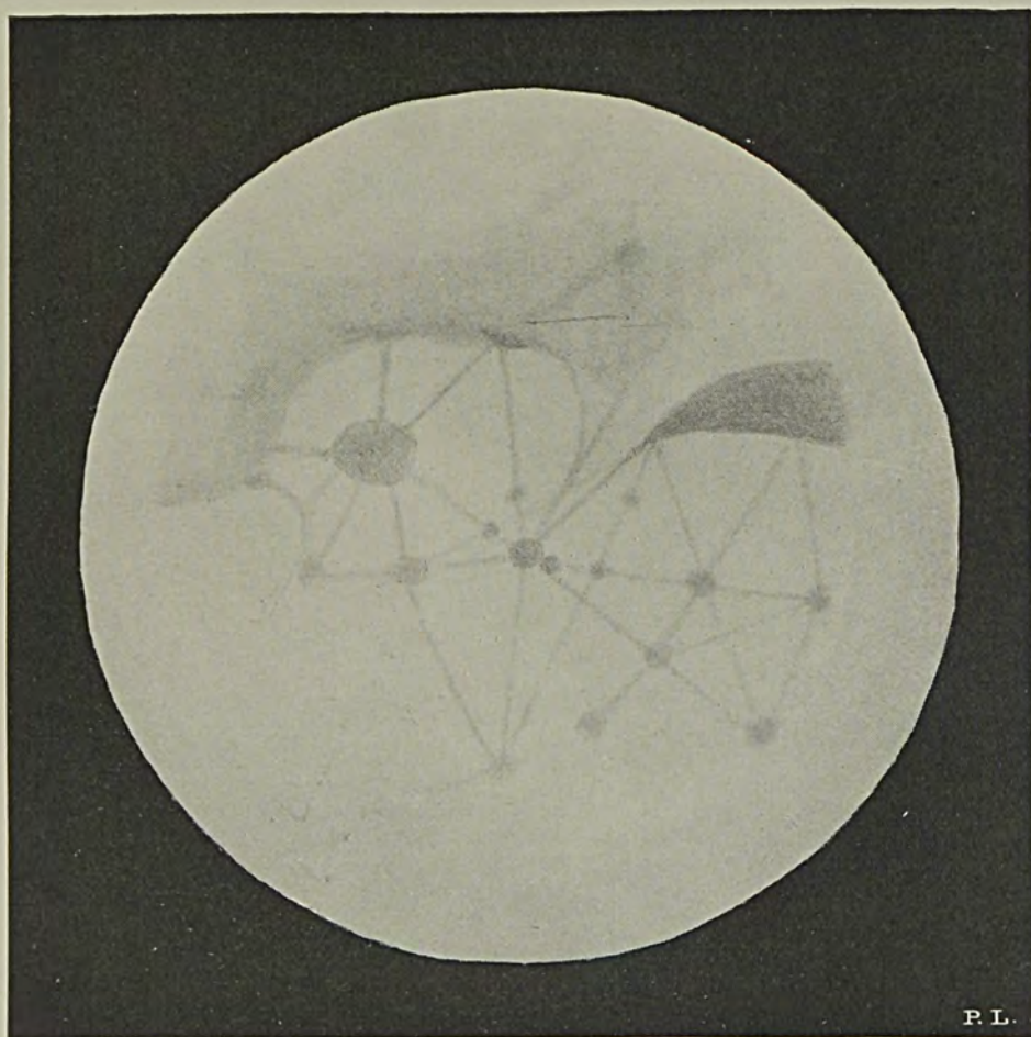
LACUS PHOENICIS NOVEMBER, 1894
