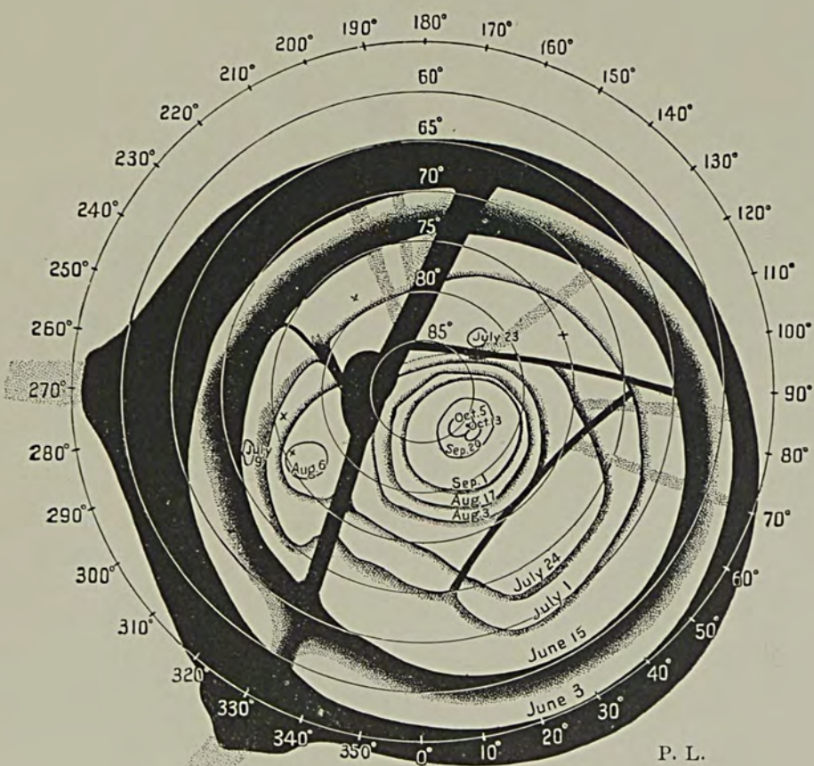
MAP OF THE SOUTH POLE OF MARS SHOWING THE POLAR CAP AND ITS CHANGES IN 1894
