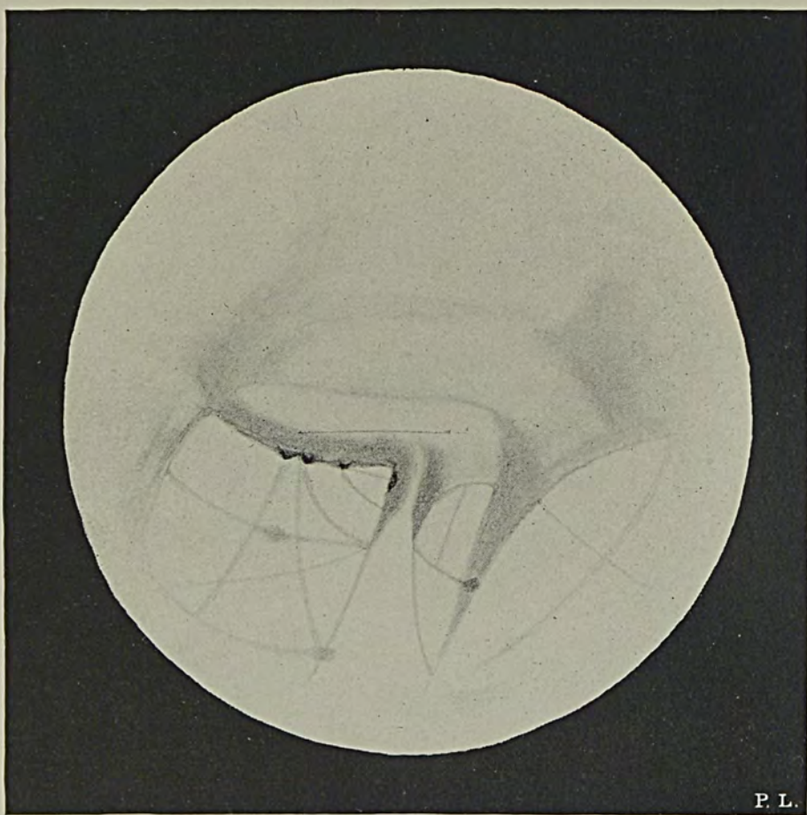
FASTIGIUM ARYN OCTOBER, 1894
