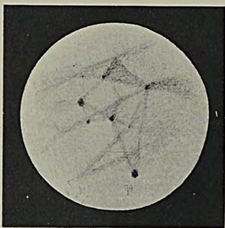
FIG. I. Nov. 14. Long. cent. 114^{\circ} Seeing 4 to 8. Diam. 17''.9
