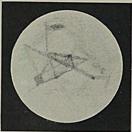
FIG. I. Nov. 26. Long. cent. 314^{\circ} Seeing 2 to 6. Diam. 15''.8
