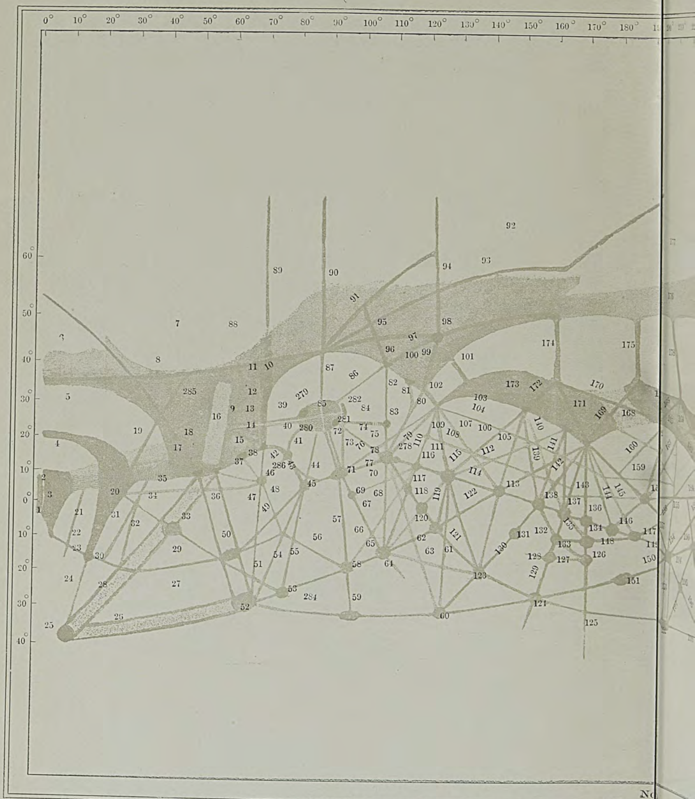
MAP OF MARS on Mercator Projection
